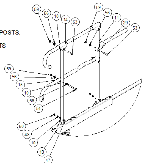
DETAIL B ACTUATORS MOUNT (LH SHOWN)
