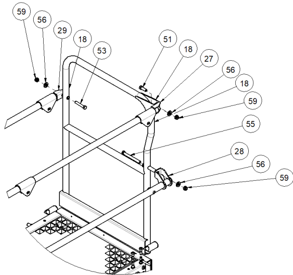
DETAIL G REAR GATE MOUNT
