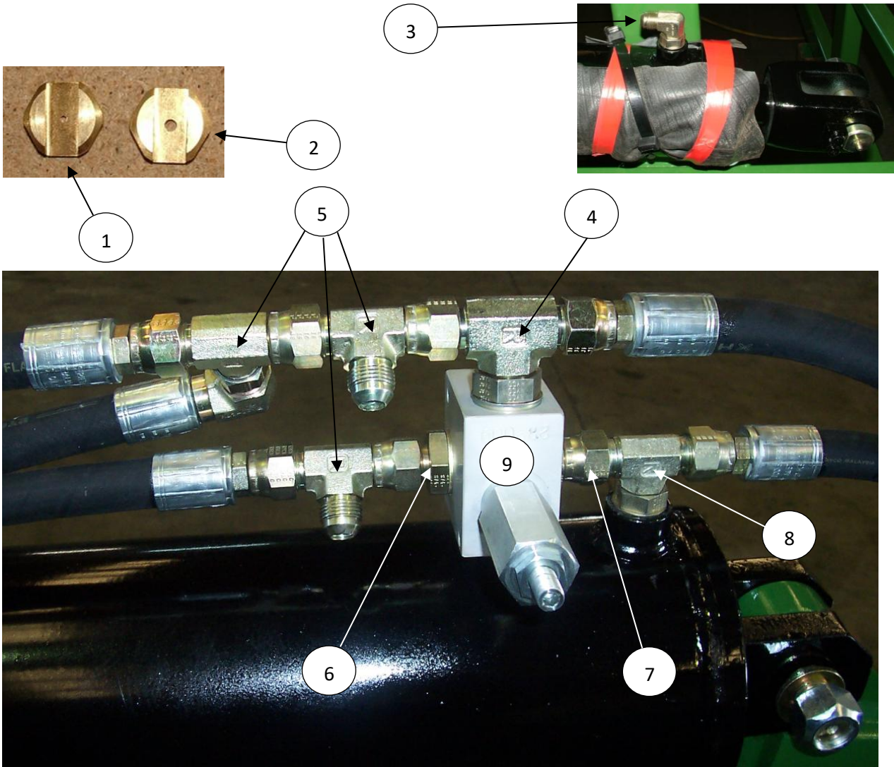
Flow Restrictor fitted grove side down at rod end
