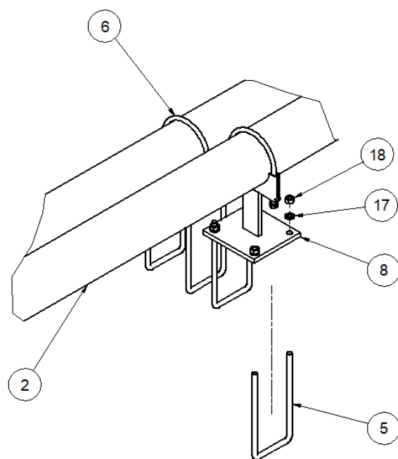
DETAIL A
