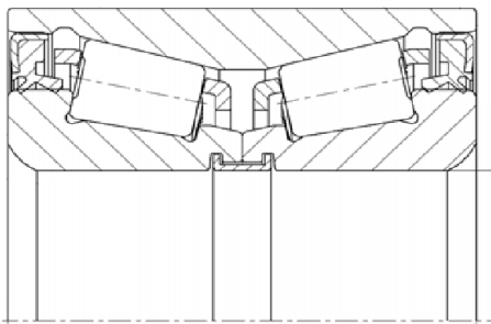
(Bearing cross section view)
