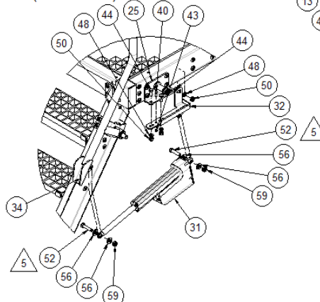
DETAIL B ACTUATORS MOUNT (LH SHOWN)
