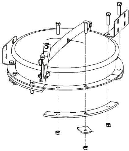
Tank Lid Assy with Brackets Part # 15061
