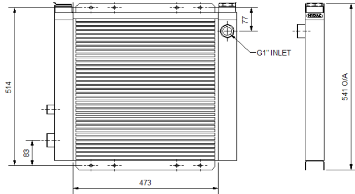
27106 Heat Exchanger
