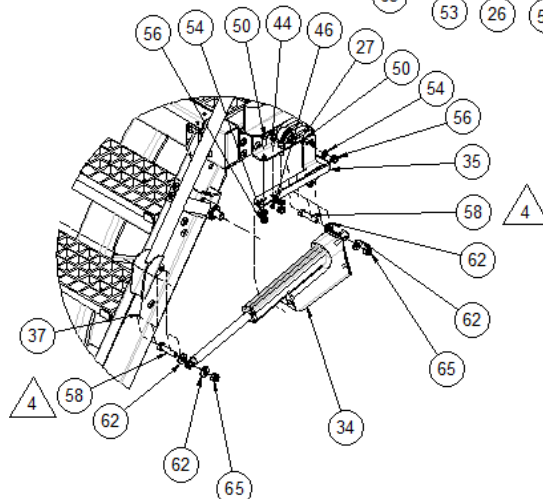
DETAIL B ACTUATORS MOUNT
