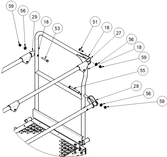
DETAIL G REAR GATE MOUNT
