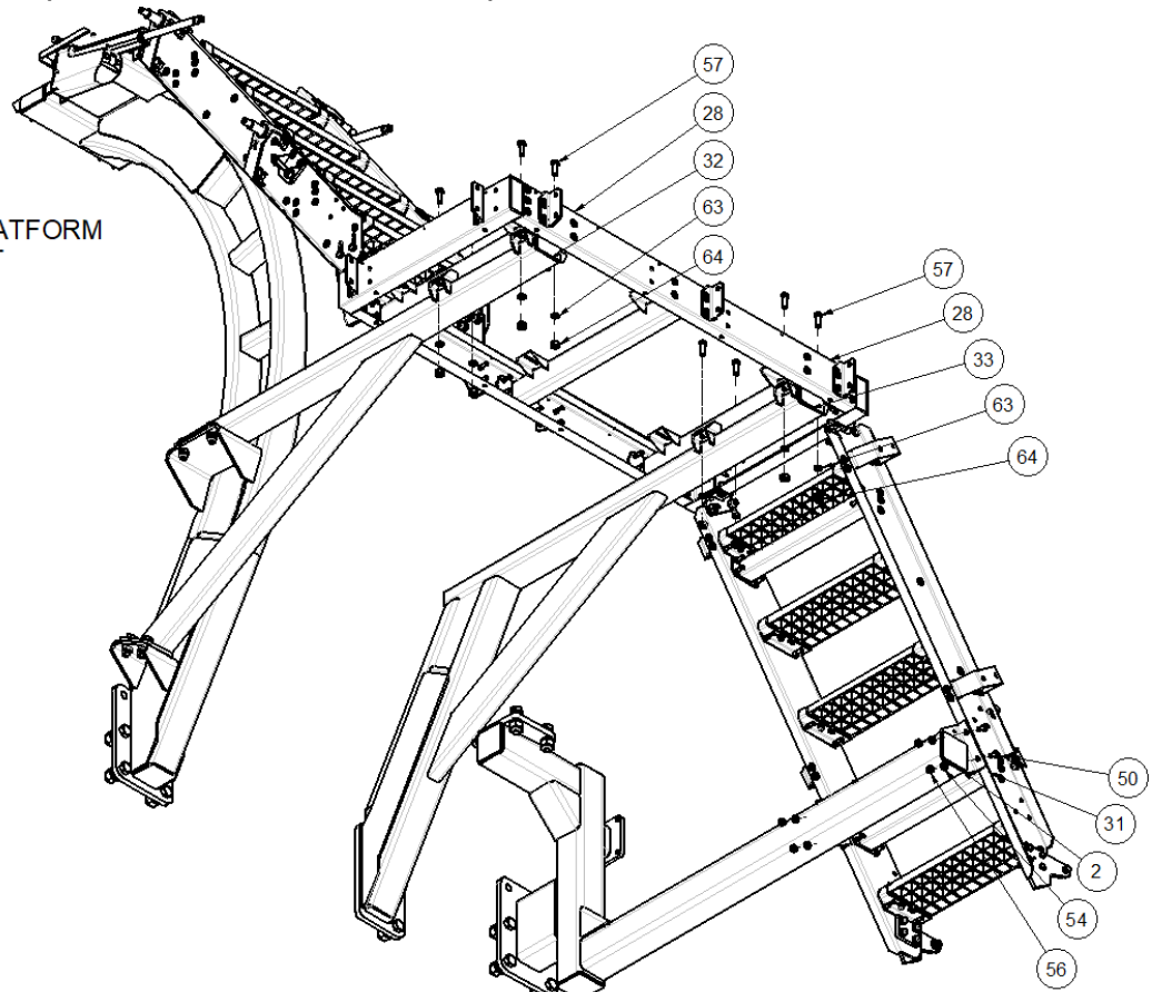
DETAIL A FRONT INTERNAL POSTS, HANDRAILS AND KICKPLATE MOUNTS
