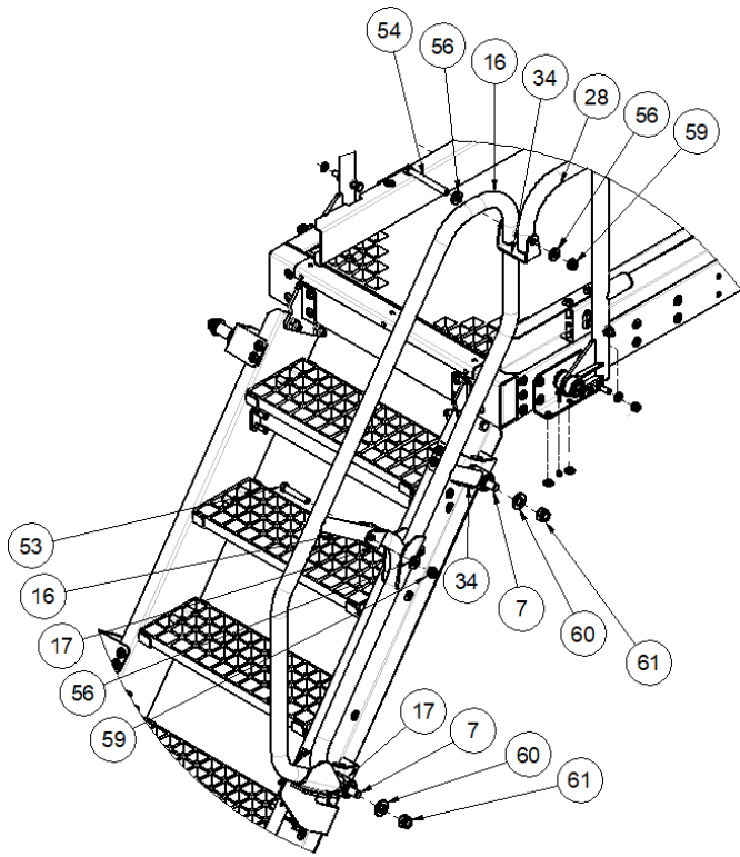
DETAIL E UPPER LADDER HANDRAIL MOUNT
