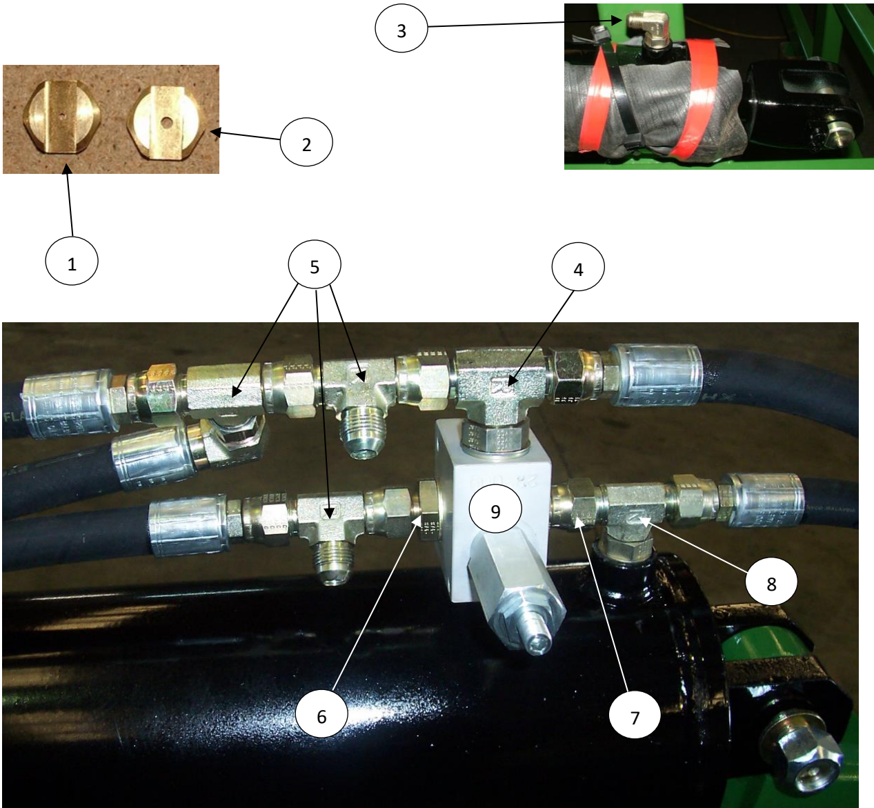
Flow Restrictor fitted grove side down at rod end
