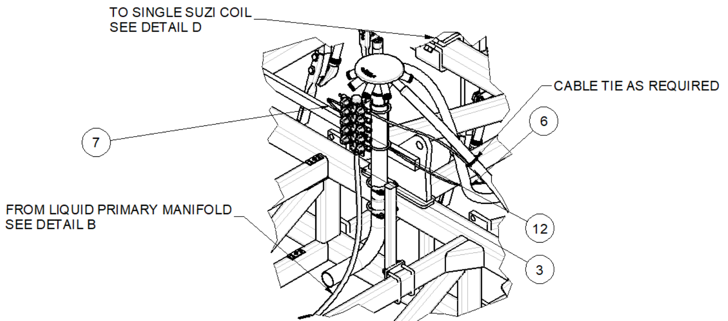
DETAIL C TYPICAL LIQUID MANIFOLD ASSEMBLY
