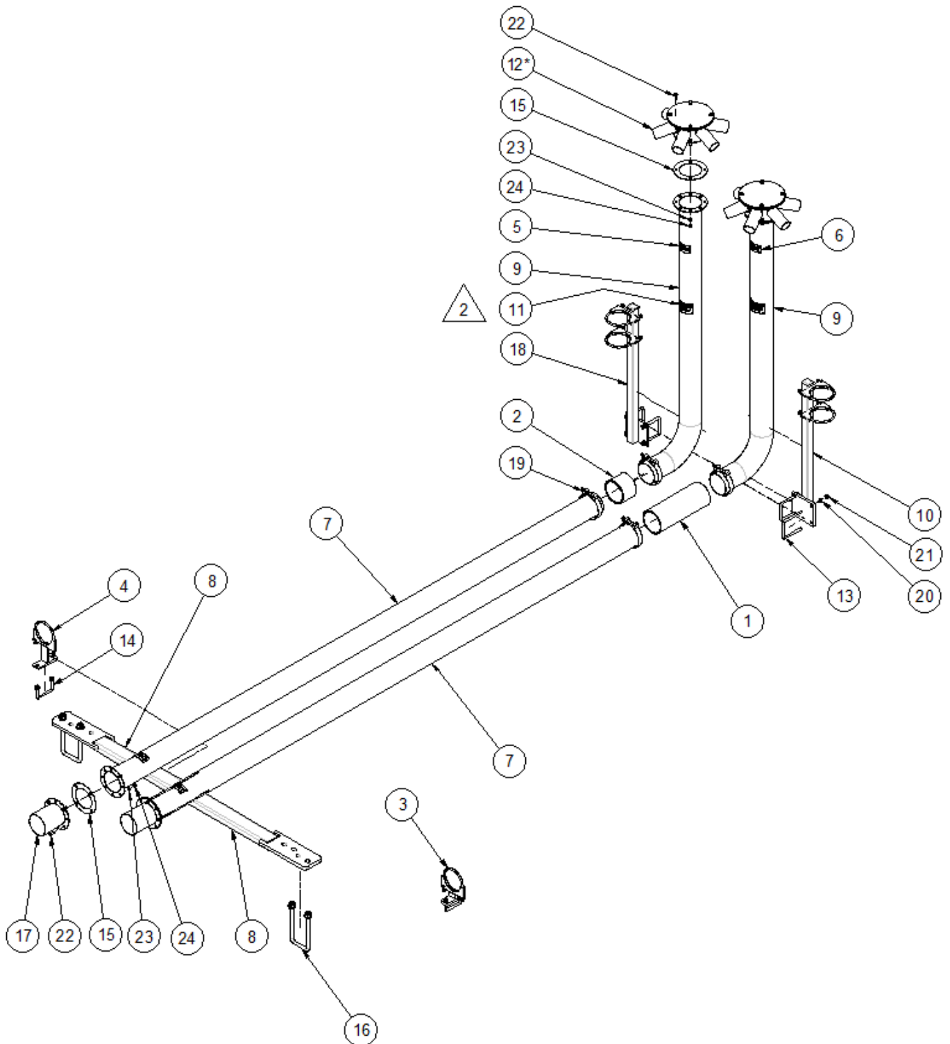
Primary Air Head Risers – Side by Side - TBT (28881 & 28886)
